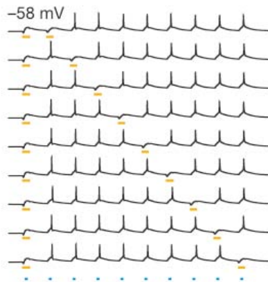
A two-second sequence of flashes (blue bars) of blue light triggers electrical spikes in a nerve cell with ChR2 photoreceptors, except when a simultaneous flash of yellow (orange bar) inhibits the cell’s activity.
